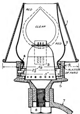
Fig. 3323. Locomotive Cab Lamp. Pennsylvania Railroad.
